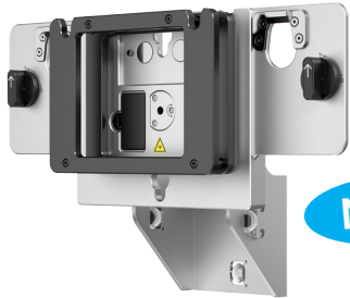
Mounting Plate MA600RAP
