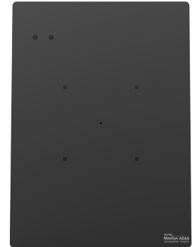
Radar Calibration Plate CSC0602/02
