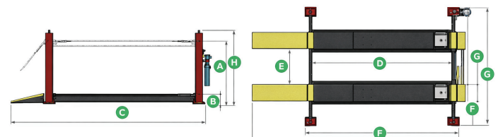
4-POST ALIGNMENT
