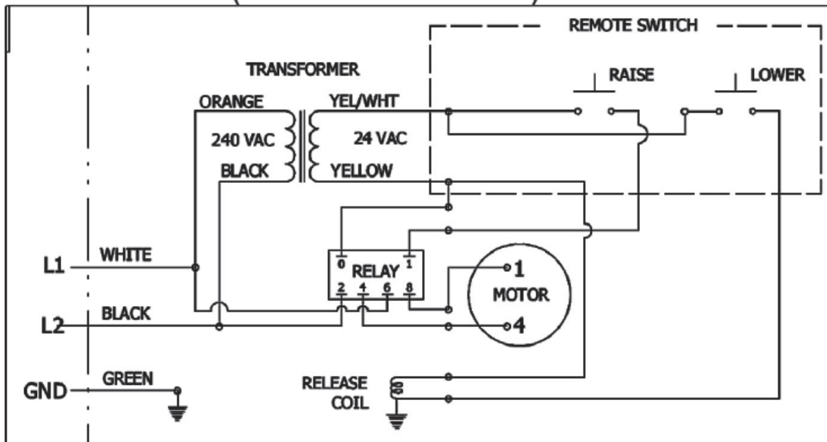
PLT-6 Wiring Diagram 208-230VAC, 1 Ph
