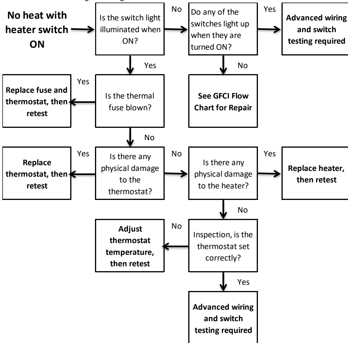
No Heat Troubleshooting Flow Diagram:
