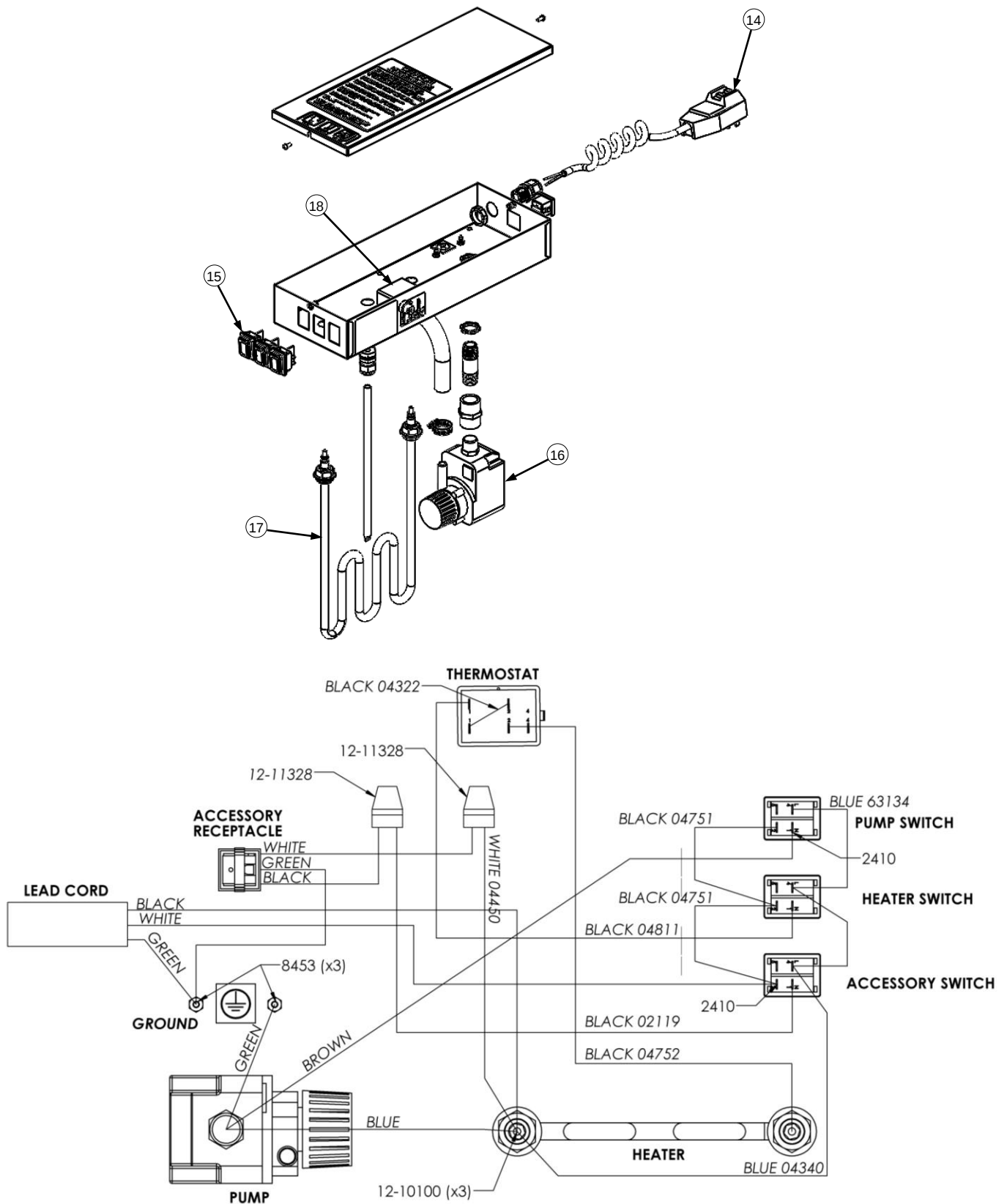
WIRING DIAGRAM
