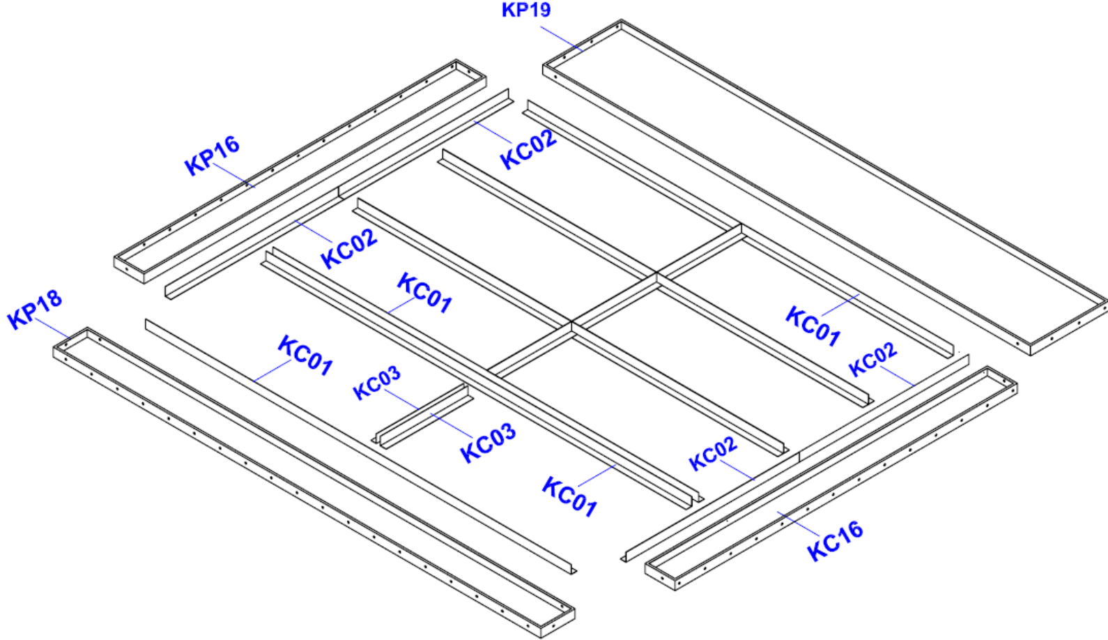
Small Intake Filter Grid – End Sections
